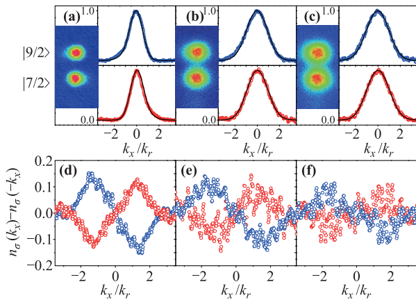
Fig. 4 Momentum distribution asymmetry as a hallmark of SO coupling: (a)–(c) time-of-flight measurement of momentum distribution for both |\uparrow\rangle (blue) and |\downarrow\rangle (red). Solid lines are theory curves. (a) k_F = 0.9k_r and T/T_F = 0.8 ; (b) k_F = 1.6k_r and T/T_F = 0.63 ; (c) k_F = 1.8k_r and T/T_F = 0.67 . (d)–(f) Plot of integrated momentum distribution n_\sigma(\mathbf{k}) - n_\sigma(-\mathbf{k}) for the case of (a)–(c).
